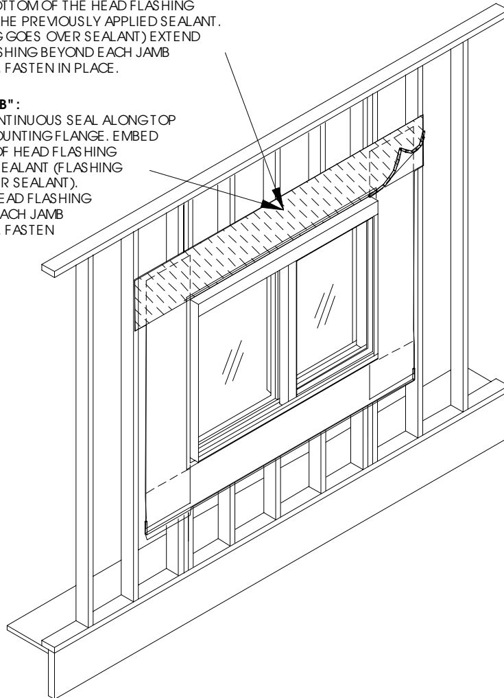
Figure 5: Head Flashing
